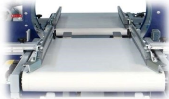
Angled idle guide roller option for 0.12" base
